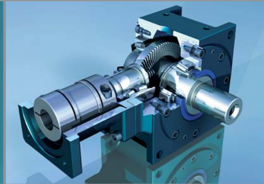
ZF-Servoplan CG Compact Gearboxes
